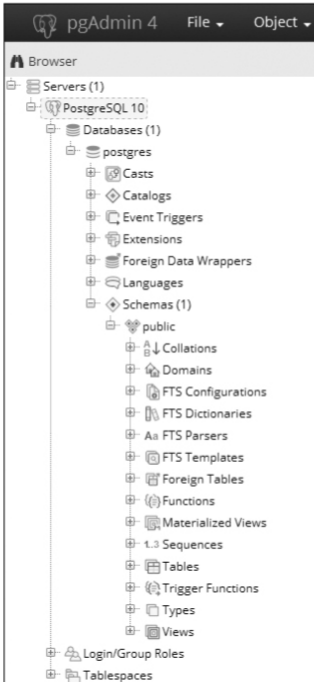
Figure 2: The pgAdmin object browser
